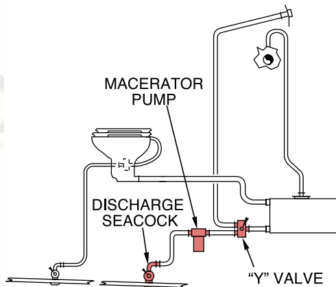
TYPICAL MACERATOR SYSTEM KC-2046
