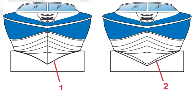
1 – Hull completely on cradle — right
