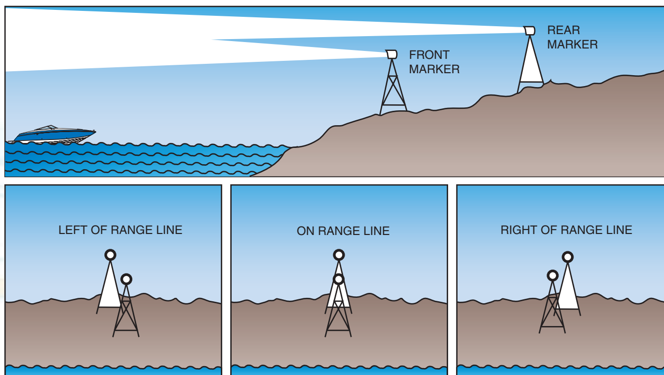
RANGE LIGHTS
