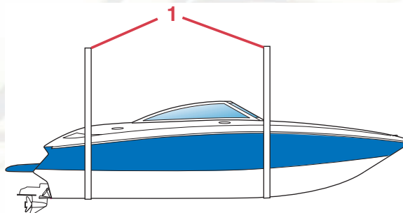
1 – Flat, wide-belting sling
